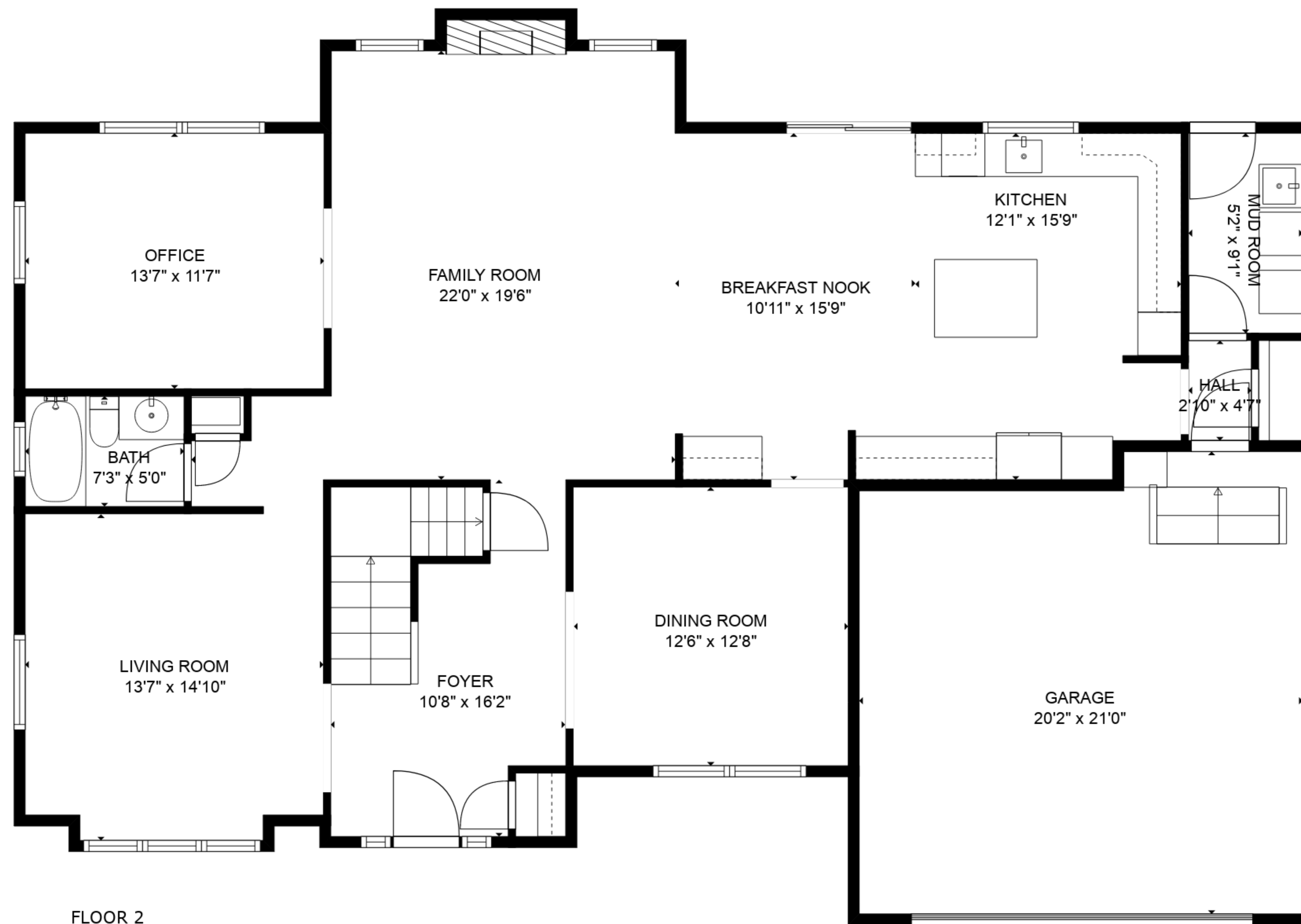
FLOOR 2
